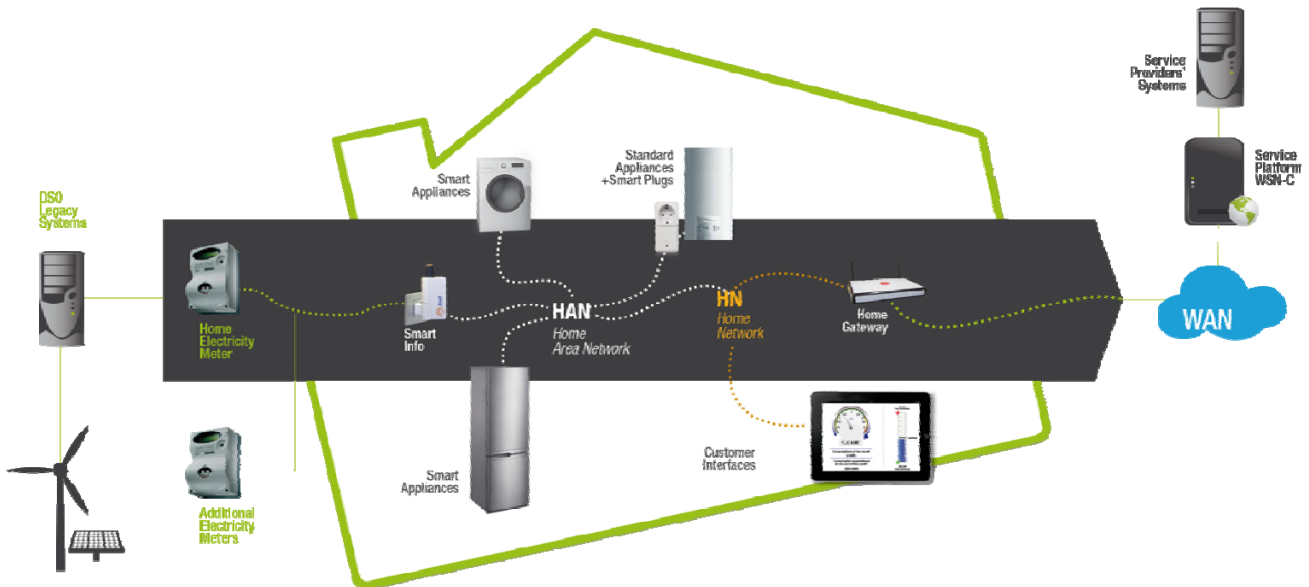
Figure 2: Energy@home architecture
